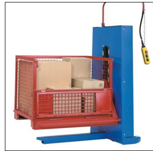
Electro-mechanical container lifter
