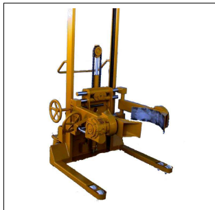
High lift stacker to grip and tilt
