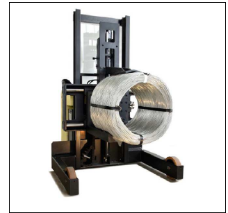
High lift stacker with straddle legs for coil transport
